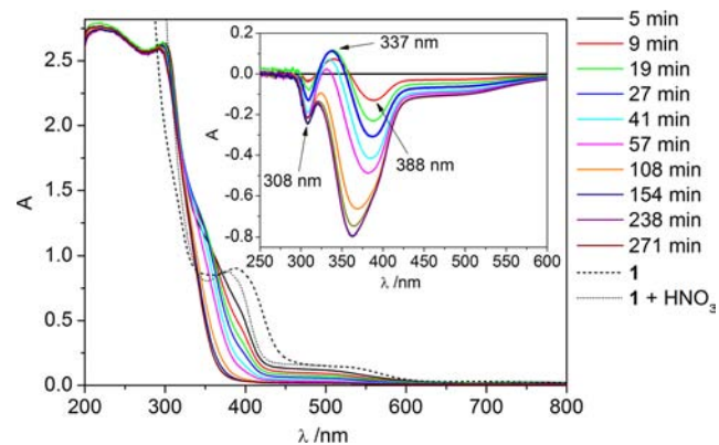
Figure 18. UV/vis spectra of acetonitrile solution of 1 ( 5 \times 10^{-5} \text{ M} ), dashed line (---); acetonitrile solution of 1 ( 5 \times 10^{-5} \text{ M} ) with HNO_3 (0.04 M, 65% aqueous), dotted line (···); solid lines illustrate the spectra of catalytic solutions in cyclooctane (0.25 M) oxidation with H_2O_2 (1.0 M, 50% aqueous) catalyzed by complex 1 ( 5 \times 10^{-5} \text{ M} ) in the presence of HNO_3 (0.04 M, 65% aqueous) in acetonitrile (total volume of the reaction solution was 5 mL), 50^\circ \text{C} . The inset shows the difference spectra taking 5 min spectrum as the basic one.
